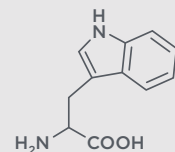
Tryptophan (Trp, W) MW: 186.21
