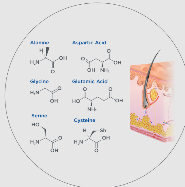
Glutamic Acid (Glu, E) MW: 129.12, pK a ~ 4.07
