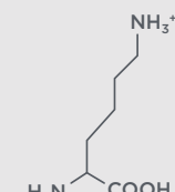
Lysine (Lys, K) MW: 128.17, pK a ~ 10.79
