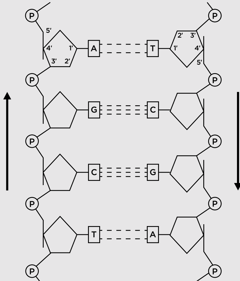
Chemical Structure of PDRN
