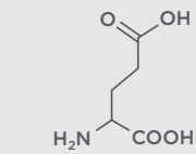
Glutamic Acid (Glu, E) MW: 129.12, pK a ~ 4.07
