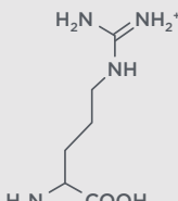
Arginine (Arg, R) MW: 156.19, pK a ~ 12.48
